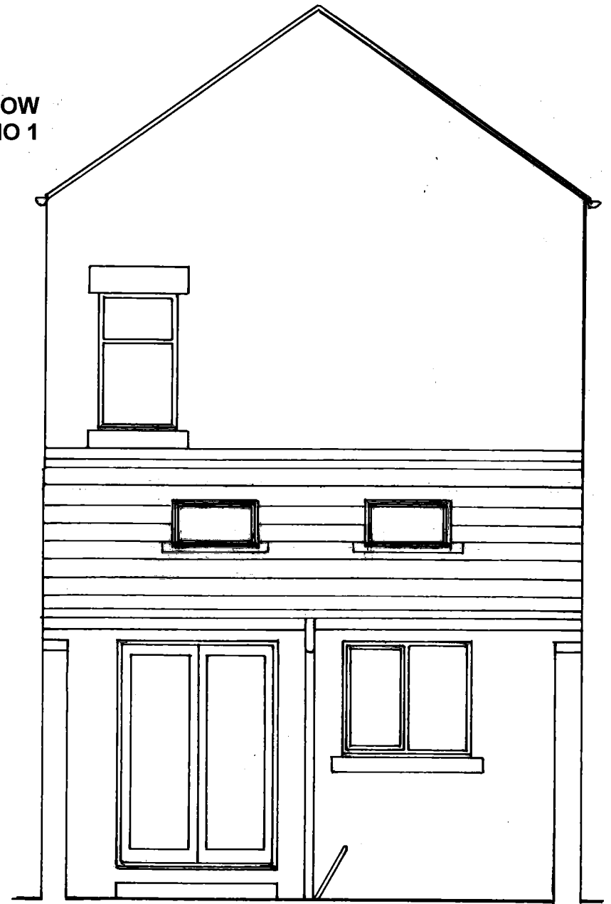
PROPOSED REAR 1:50
